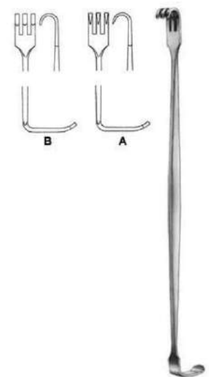
Senn-Miller PSI-5-924-16 Hooklet 16 cm
