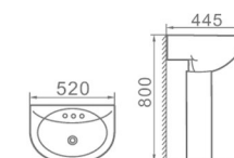
DW212 立柱盆 Pedestal Basin Size:520x445x800mm Fixing to wall with back 背靠墙式安装
