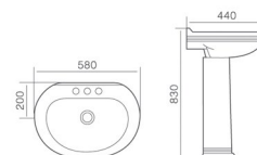
DW204 立柱盆 Pedestal Basin Size:580x440x830mm Fixing to wall with back 背靠墙式安装
