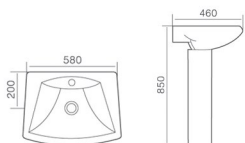
DW344 立柱盆 Pedestal Basin Size:580x460x850mm Fixing to wall with back 背靠墙式安装
