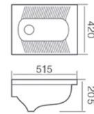
DP003 蹲便器 Squatting Pan W.C. Size:515x420x205mm Build-in platform
