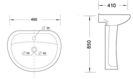
DW207 立柱盆 Pedestal Basin Size: 490x410x850mm Fixing to wall with back 背靠墙式安装
