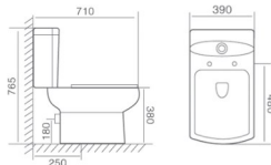
DT2044 直冲分体坐便器 Washdown Close-couched Closet Size:710x390x765mm S-trap,250mm Roughing-in 地排污口中心离墙250mm P-trap,180mm Roughing-in 横排污口中心离地180mm
