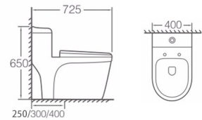
DA8075 虹吸/直冲连体坐便器 Siphonic/Washdown One-piece Toilet Size: 725x400x650mm S-trap, 250, 300, 400mm Roughing-in 地排污口中心离墙250, 300, 400mm P-trap, 180mm Roughing-in 横排污口中心离地180mm
