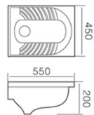
DP001 蹲便器 Squatting Pan W.C. Size:550x450x200mm Build-in platform
