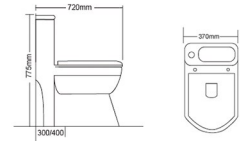
DA8304 虹吸/直冲连体坐便器 Siphonic/Washdown One-piece Toilet Size:720x370x775mm S-trap,250,300,400mm Roughing-in 地排污口中心离墙250,300,400mm P-trap,180mm Roughing-in 横排污口中心离地180mm
