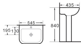
DW317 立柱盆 Pedestal Basin Size: 545x435x840mm Fixing to wall with back 背靠墙式安装
