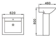
DW218 立柱盆 Pedestal Basin Size: 620x460x800mm Fixing to wall with back 背靠墙式安装
