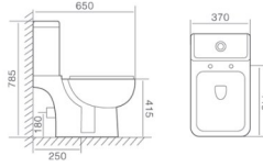
DT2040 直冲分体坐便器 Washdown Close-couched Closet Size:650x370x785mm S-trap,250mm Roughing-in 地排污口中心离墙250mm P-trap,180mm Roughing-in 横排污口中心离地180mm
