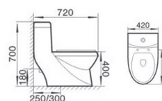
DA8069 直冲连体坐便器 Washdown One-piece Toilet Size:720x420x700mm S-trap,250,300mm Roughing-in 地排污口中心离墙250,300mm P-trap,180mm Roughing-in 横排污口中心离地180mm
