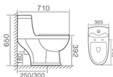
DA8018 直冲连体坐便器 Washdown One-piece Toilet Size:710x365x650mm S-trap,250,300mm Roughing-in 地排污口中心离墙250,300mm P-trap,180mm Roughing-in 横排污口中心离地180mm
