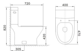
DT2604 虹吸分体坐便器 UPC WaterSense Siphonic Close-couched Closet Size:720x400x820mm S-trap,305mm Roughing-in 地排污口中心离墙305mm
