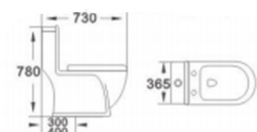
DA8111 虹吸/直冲连体坐便器 Siphonic/Washdown One-piece Toilet Size: 730x365x780mm S-trap, 250, 300, 400mm Roughing-in 地排污口中心离墙250, 300, 400mm P-trap, 180mm Roughing-in 横排污口中心离地180mm
