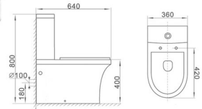
DT2512 直冲分体坐便器 WaterMark Washdown Close-couched Closet Size:640x360x800mm P-trap,180mm Roughing-in 横排污口中心离地180mm
