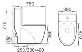
DA8001 虹吸/直冲连体坐便器 Siphonic/Washdown One-piece Toilet Size:750x390x775mm S-trap,250,300,400mm Roughing-in 地排污口中心离墙250,300,400mm P-trap,180mm Roughing-in 横排污口中心离地180mm
