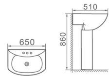
DW219 立柱盆 Pedestal Basin Size: 650x510x860mm Fixing to wall with back 背靠墙式安装
