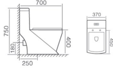
DA8114 直冲连体坐便器 Washdown One-piece Toilet Size:700x370x750mm S-trap,250mm Roughing-in 地排污口中心离墙250mm P-trap,180mm Roughing-in 横排污口中心离地180mm
