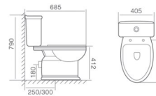
DT2004 直冲分体坐便器 Washdown Close-couched Closet Size:685x405x790mm S-trap,250,300mm Roughing-in 地排污口中心离墙250,300mm P-trap,180mm Roughing-in 横排污口中心离地180mm
