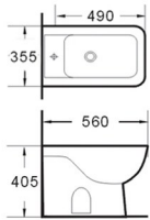
DF040 妇洗器 Bidet Size:560x355x405mm Fixing to wall with back 背靠墙式安装
