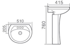
DW202 立柱盆 Pedestal Basin Size: 510x415x760mm Fixing to wall with back 背靠墙式安装
