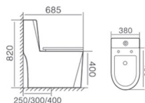
DA8007 虹吸/直冲连体坐便器 Siphonic/Washdown One-piece Toilet Size:685x380x820mm S-trap,250,300,400mm Roughing-in 地排污口中心离墙250,300,400mm P-trap,180mm Roughing-in 横排污口中心离地180mm
