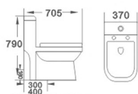
DA8061 虹吸/直冲连体坐便器 Siphonic/Washdown One-piece Toilet Size:705x370x790mm S-trap,250,300,400mm Roughing-in 地排污口中心离墙250,300,400mm P-trap,180mm Roughing-in 横排污口中心离地180mm
