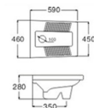
DP006-S 蹲便器 Squatting Pan W.C. Size:590x460x280mm Build-in platform
