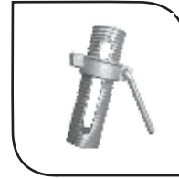
Prop Sleeve Application: For Light/Heavy duty Props system component Weight: 1 kg to 2 kg Pipe thicknes : 3mm/4mm
