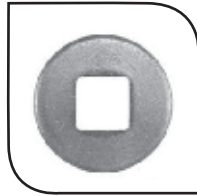
Round washer for Square Spigot Size : 31 mm x 31 mm SHS Finish : GI and MS Thickness : 2.5 mm
