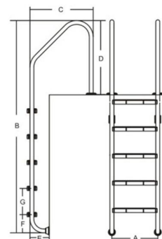
SL 型不锈钢扶梯 SL Series Stainless Steel Pool Ladder
