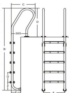
SF 型不锈钢扶梯 SF Series Stainless Steel Pool Ladder
