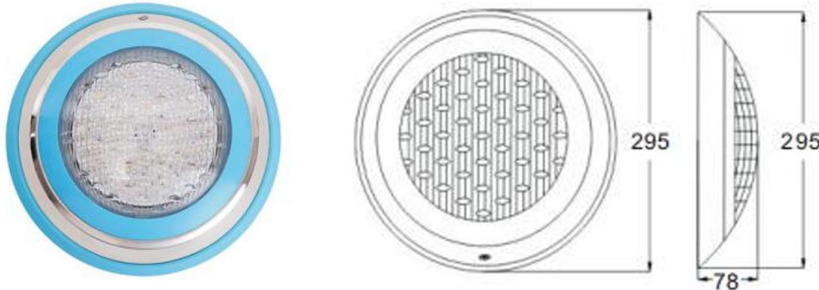
MC002 wall mounted type pool light
