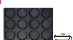
Alu.Steel 400x600x32mm
