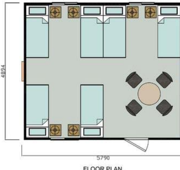
FLOOR PLAN
