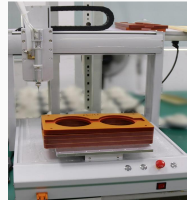
Dispensing Machine
