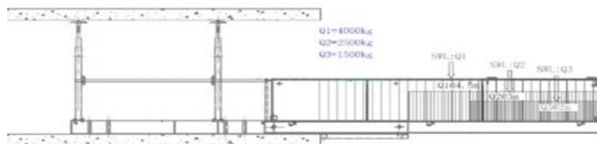
Safe Working Load Distribution
