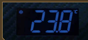
LED Display
