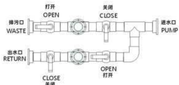
反冲洗状态 Backwashing state
