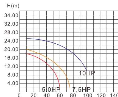
铸铁泵性能曲线图 Performance chart
