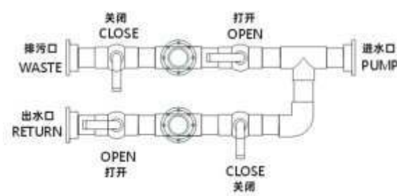
正常过滤状态 Normal filter state
