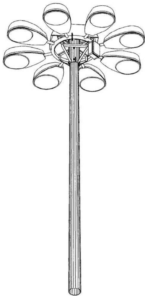
Lantern carriage with 8 No. symmetrically arranged lanterns
